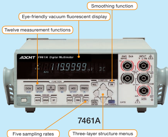
Front Panel
