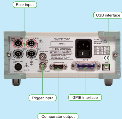
Rear Panel
